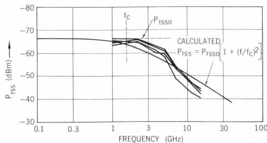
Fig. 8. Measured frequency response of typical hpa 2350 series diodes for tangential signal power P_{TSS} . Measured at 27 \mu A bias with 10^7 - 5 Hz video bandwidth.
