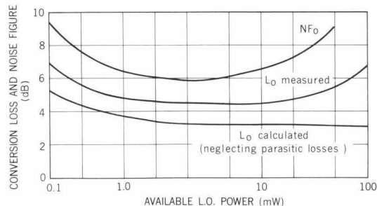
Fig. 6. Conversion loss ( L_0 ) and noise figure ( NF_0 ) for typical hpa 2350 series diodes vs. LO available power. f_0 = 2 GHz, IF = 30 MHz, NF_{IF} = 1.5 dB.
