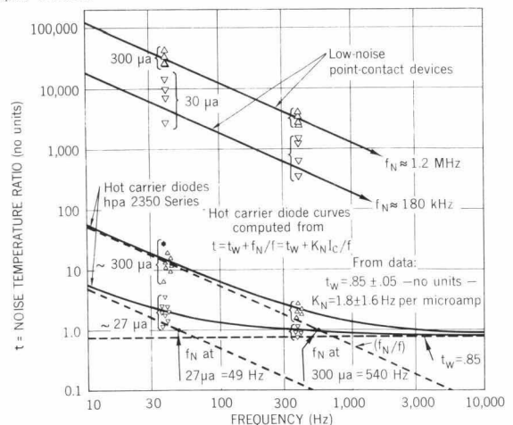
Fig. 2. Spectral density of relative noise power (or "noise temperature ratio") for hot carrier and point contact devices.
