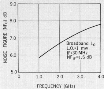
Fig. 8. Noise figure ( NF_0 ) vs. frequency for typical hpa 2350 series diode. Broadband L_0 test conditions with LO = 1 mW, IF = 30 MHz, NF_{IF} = 1.5 dB.
