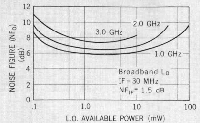
Fig. 9. Noise figure vs. LO available power for a typical hpa 2350 series diode. Broadband L_0 , IF = 30 MHz, NF_{IF} = 1.5 dB.
